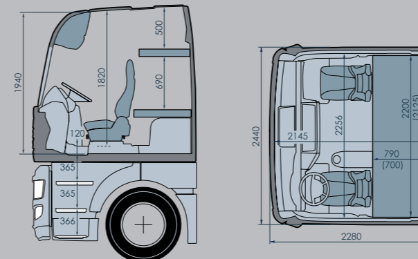
2.8 TGX vehicle portfolio (5/5) 驾驶室
